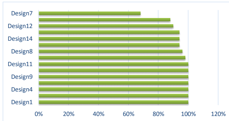
Chart 2 percentage of mean and respondents' interaction with 15 designs
