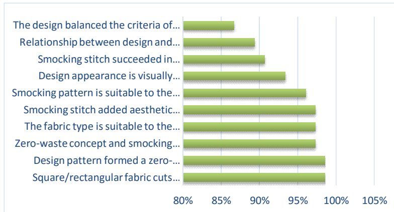
Chart 1 percentage of mean and respondents' interaction with questionnaire items.
